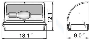
HLF-400HSW-S
