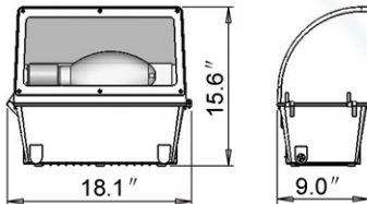
HLF-400HSW-S
