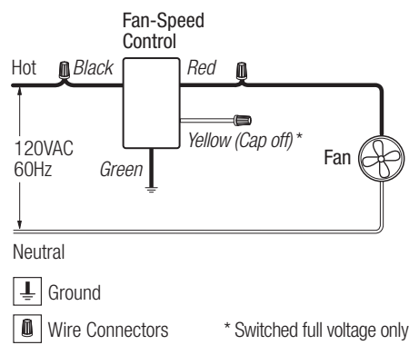
Wiring Diagram 4 Single-Pole Wiring, Fan Only
