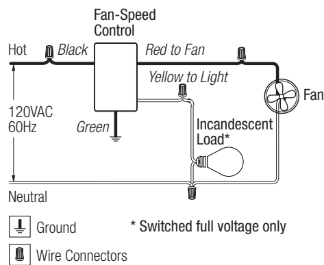
Wiring Diagram 5 Single-Pole using Fan/Light
