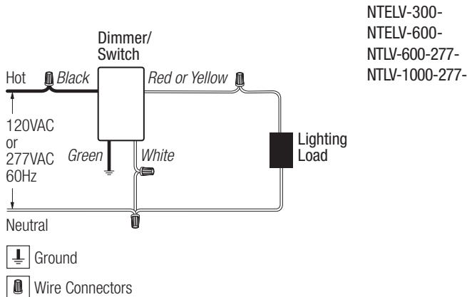
Wiring Diagram 3 Single-Pole Wiring
