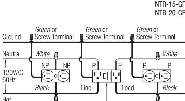
GFCI Receptacle (15A Shown)
