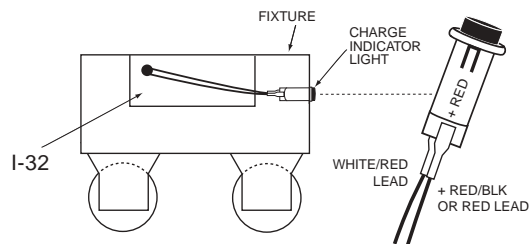
Illustration 2 Strip Fixture
