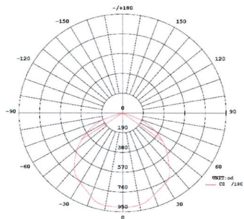
Luminous Intensity Light Distribution Diagram 100°
