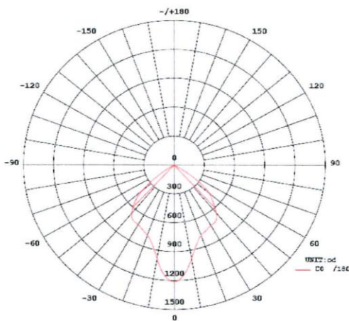
Luminous Intensity Light Distribution Diagram 50°
