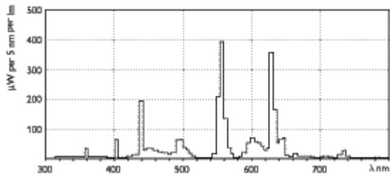
TL5 HE/840
