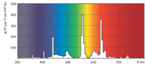
TL5 HE/840
