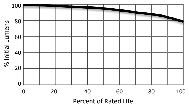
Lumen Maintenance
