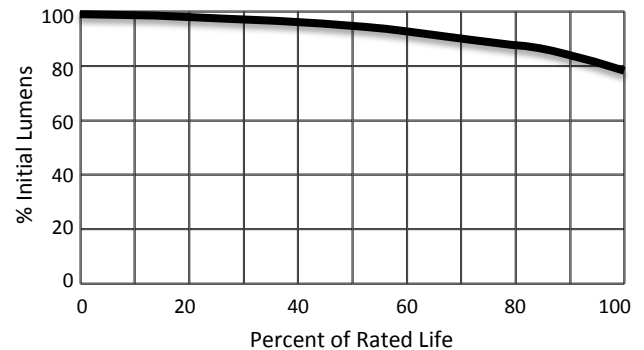
Lumen Maintenance
