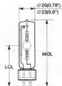
G12 Base
