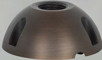
CAST BRASS DOME BASE MATTE BRONZE FINISH DIA. 2-3/4" CENTER HOLE 1/2" NPT FEMALE B2014
