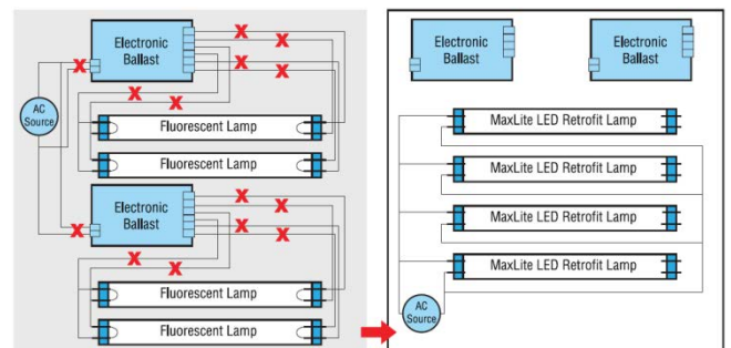
Figure 6. Retrofit with Three/Four Lamps and Two Ballasts
