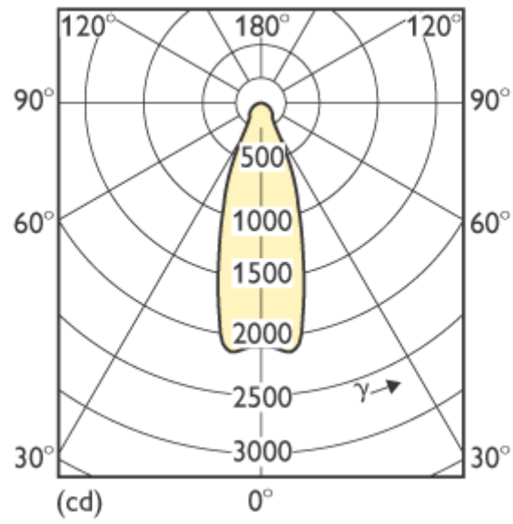
CDM-i 25W/830 40D
