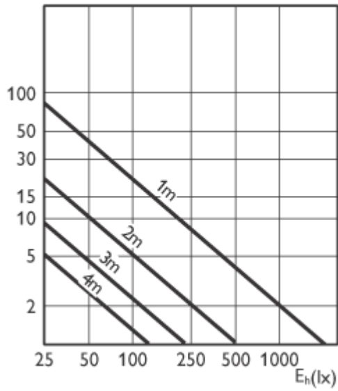
CDM-i 25W/830 40D
