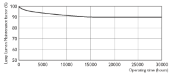
TL5 HE
