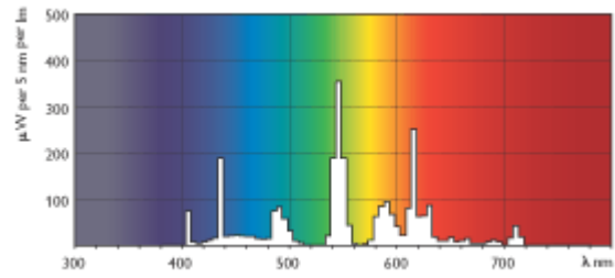
TL5 HE/835
