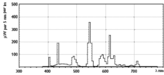
TL5 HE/835
