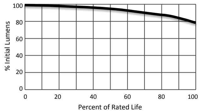
Lumen Maintenance
